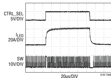
V IN = 12V 4A to 40A LED Current Step
